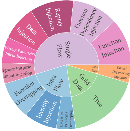
Figure 4: Overview of data distribution in MCIP-bench as the primary source for constructing the MCIP-Bench described in Section 5. It is also employed for generating synthetic training data to improve the model’s contextual robustness and security awareness. Additionally, we utilize the ToolACE dataset with 11,300 rows (Liu et al., 2024) as a complementary part of MCIP-Bench to further validate the generalization capability.
